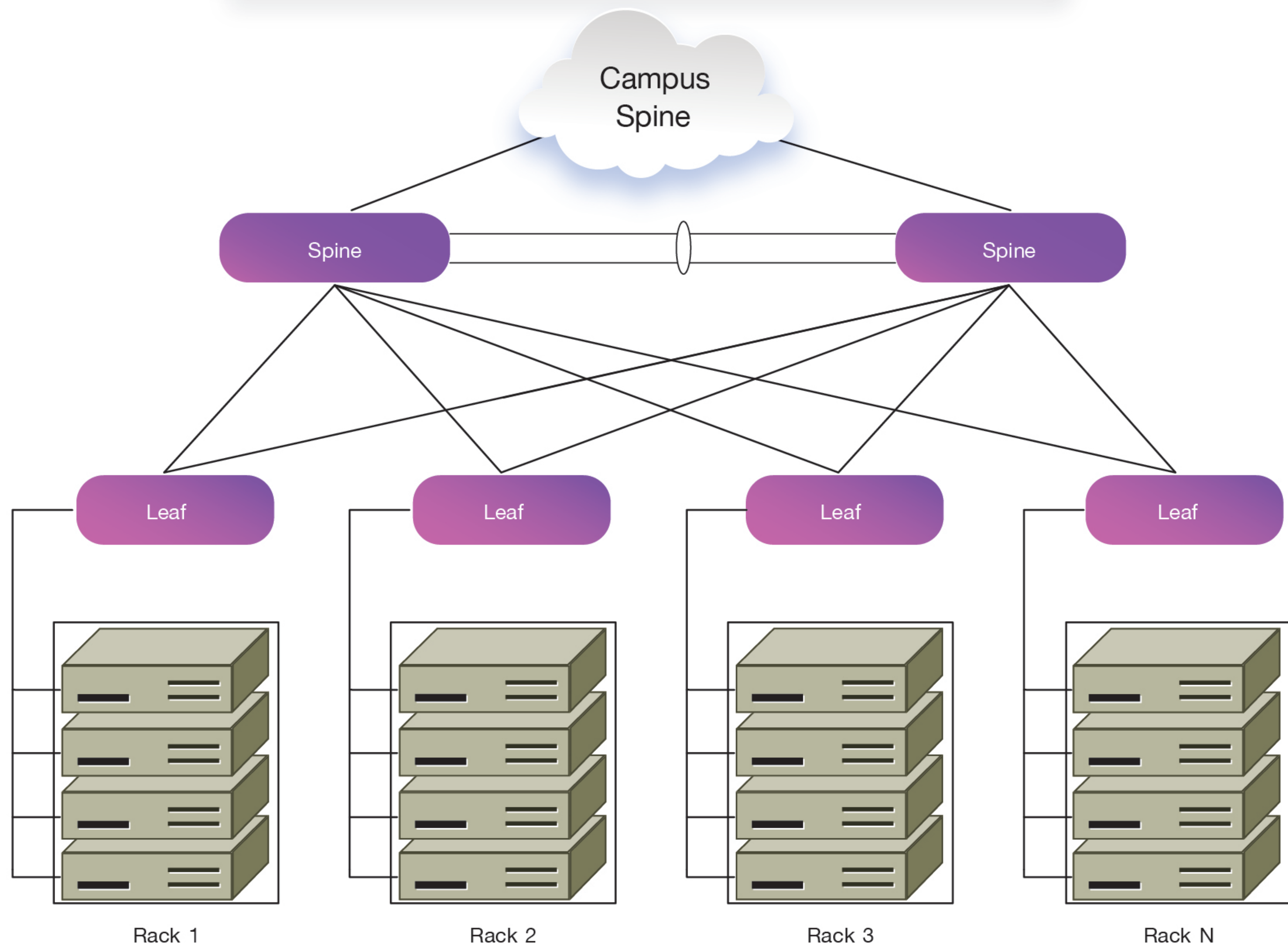
Two-Tier Data Center Network Architecture
