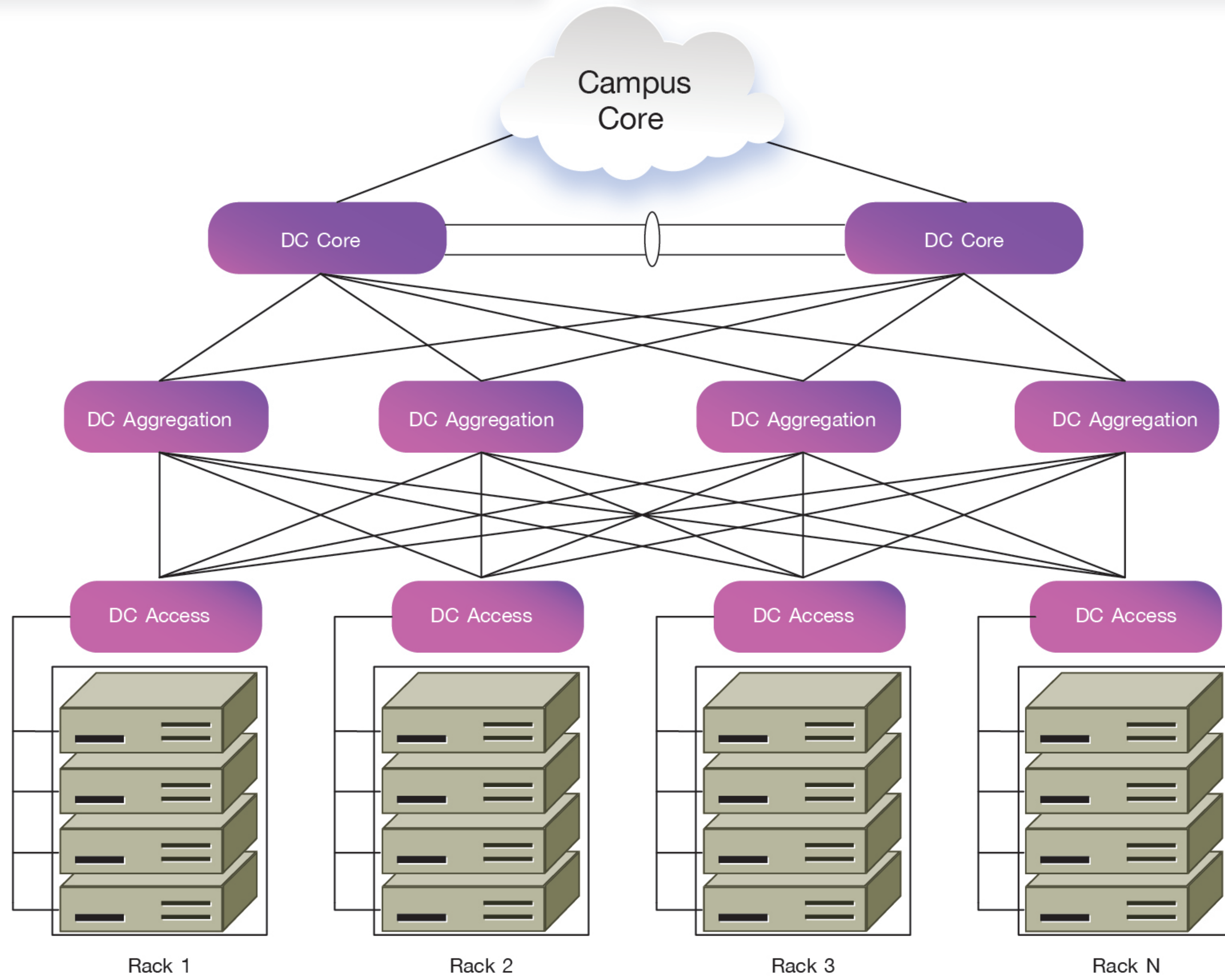
Traditional 3-Tier Network Architecture
